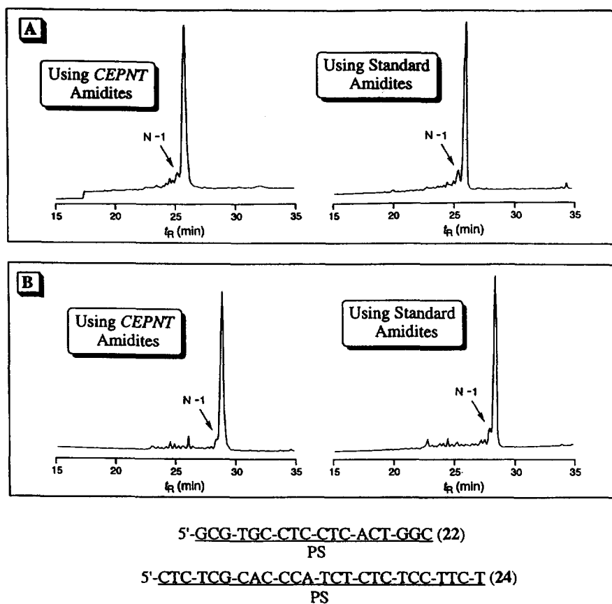
Fig. 6. Comparative CE profiles of crude 22 (18-mer) ( Panel A ) and crude 24 (25-mer) ( Panel B ) prepared using PNT and normal amidites respectively.
