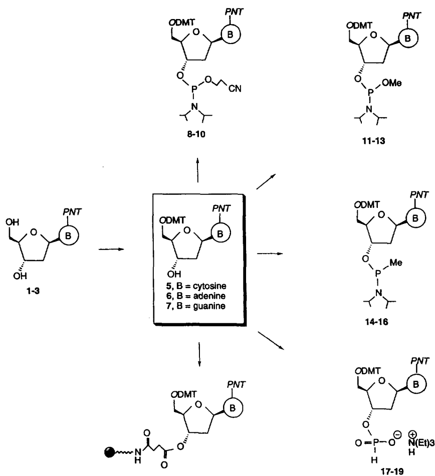
Scheme 2. Synthesis of CEPNT , MEPNT , MPNT , and H -phosphonate monomer synthons and CPG-anchored PNT nucleosides.
