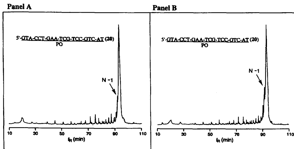
Fig. 4. Ion-exchange chromatographic profiles of crude 20 prepared using CEPNT amidites (Panel A) and that prepared using standard amidites (Panel B).
