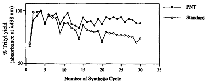
Fig. 5. Step-wise trityl monitoring during the synthesis of 25.
