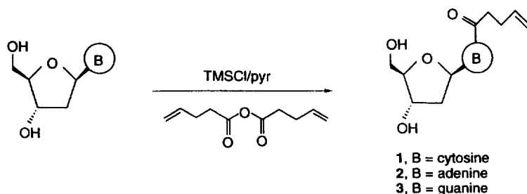
Scheme 1: Synthesis of PNT nucleosides
