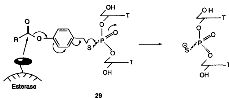
Fig. 9. Esterase-mediated bioreversibility of acyloxyaryl derivative of oligonucleotide
